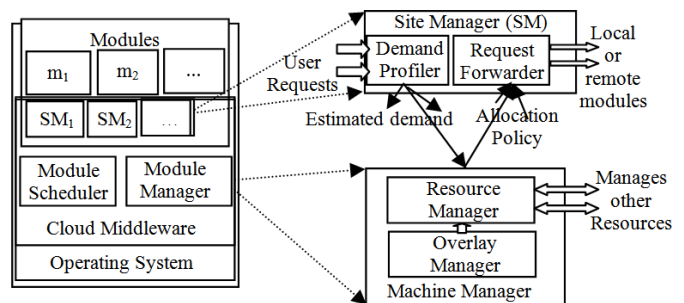
Fig. 2: Middleware Resource Allocation Architecture [32]
